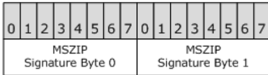
Figure 1: Figure 1: MSZIP signature
