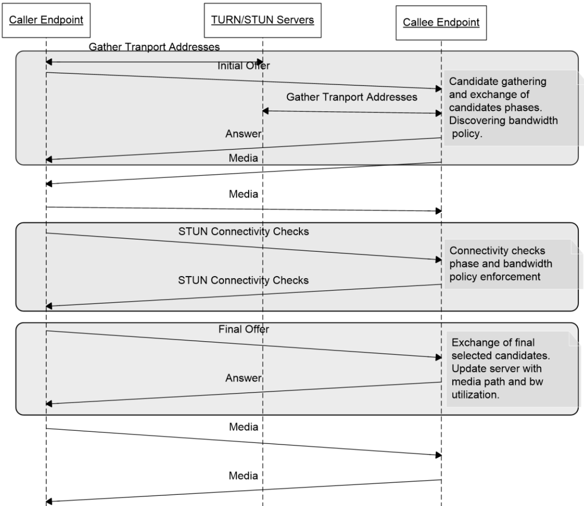
Figure 2: ICE sequence diagram
