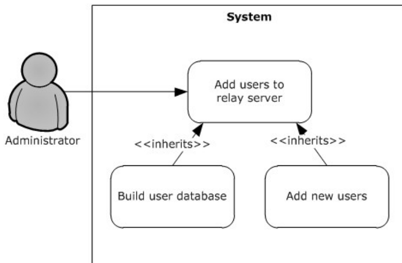
Figure 23: Process for adding users to a relay server
