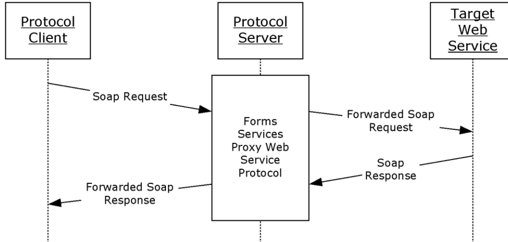
Figure 1: Protocol workflow
