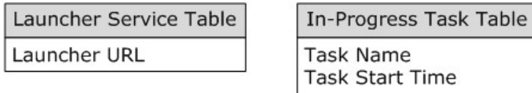
Figure 3: Tables that the IHtmlTrLoadBalancer interface maintains
