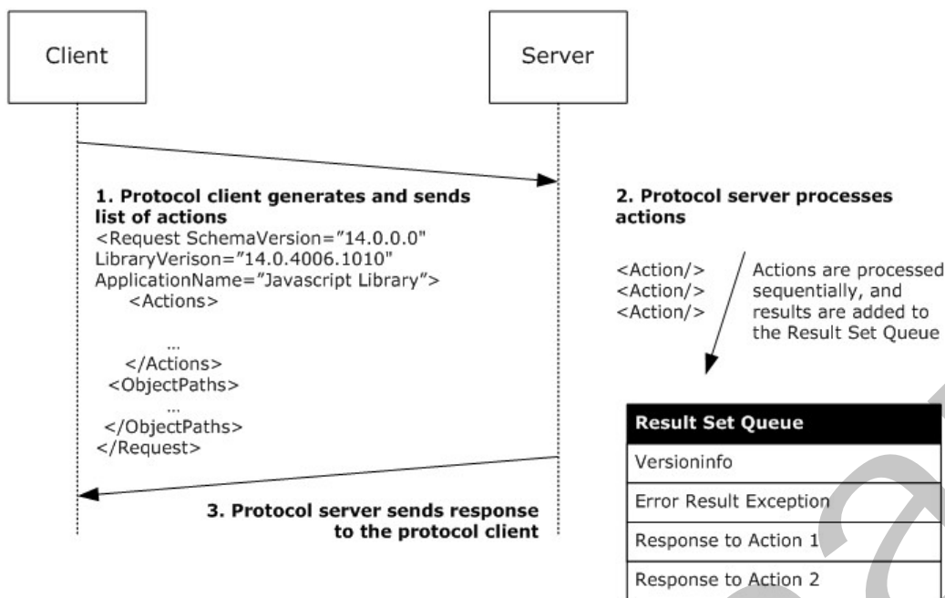
Figure 1: Overview of a request/response sequence
