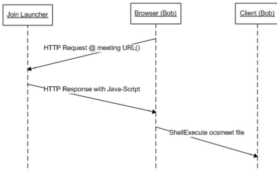
Figure 3: Simple Join
