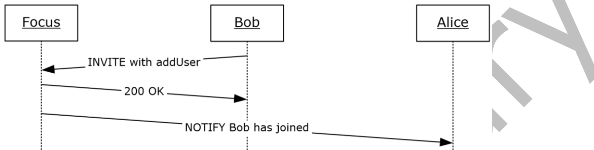
Figure 7: Joining a conference
