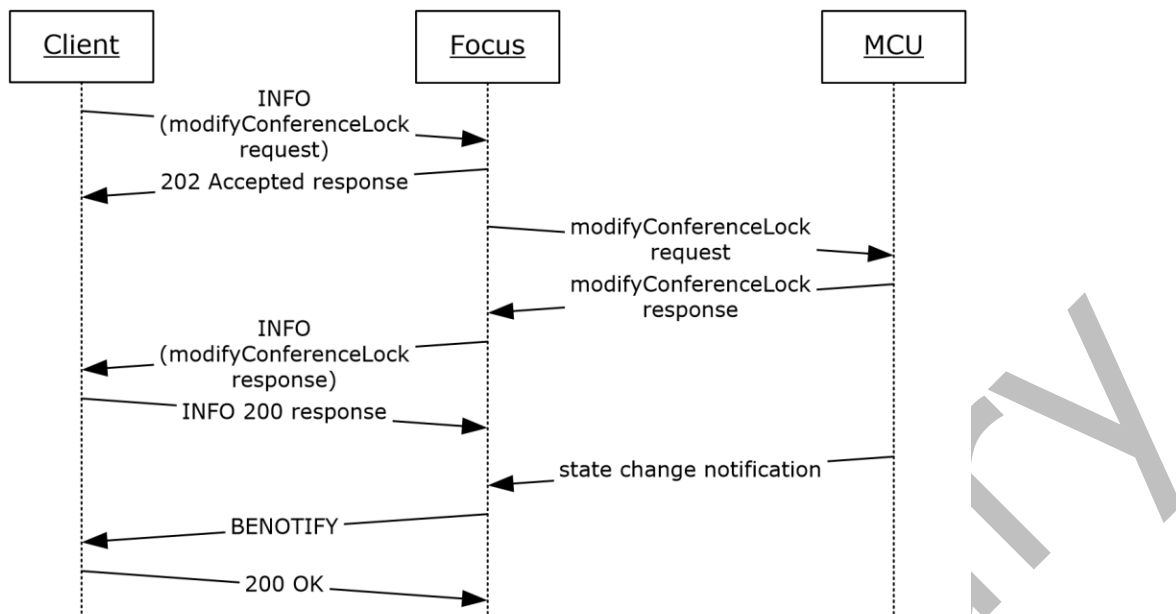
Figure 12: modifyConferenceLock call flow
