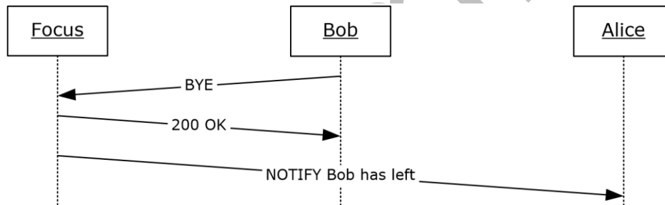
Figure 9: Leaving a conference
