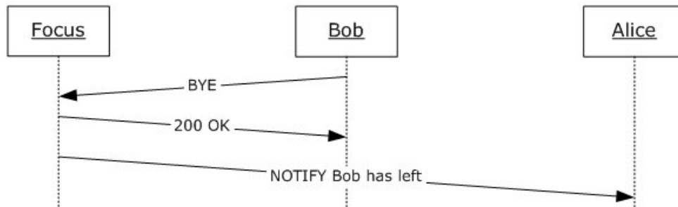
Figure 15: Leaving a conference
