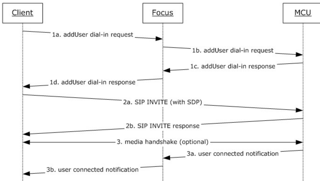
Figure 23: Connecting a Participant to an MCU
