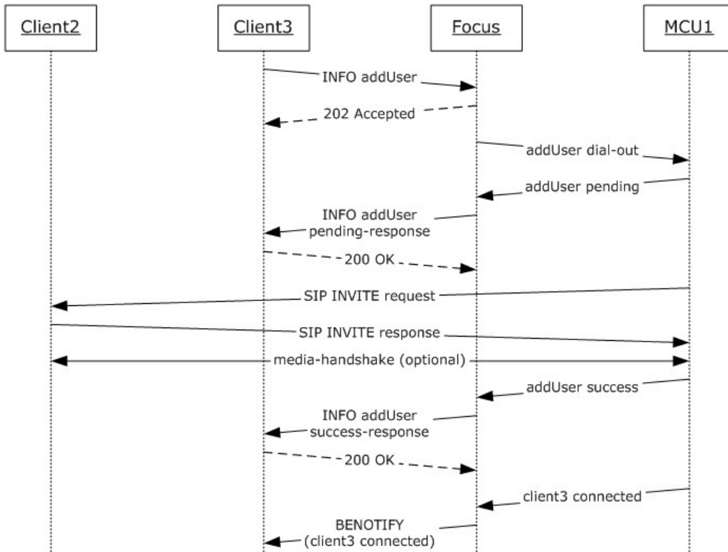
Figure 22: Connecting a Participant to an MCU
