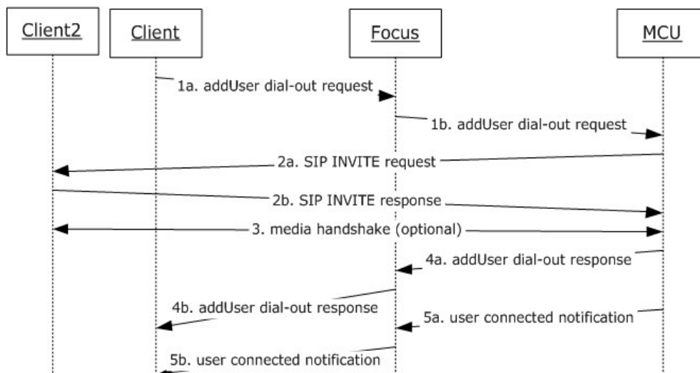
Figure 10: addUser Dial-out call flow
