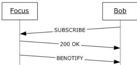
Figure 16: Establishing a subscription
