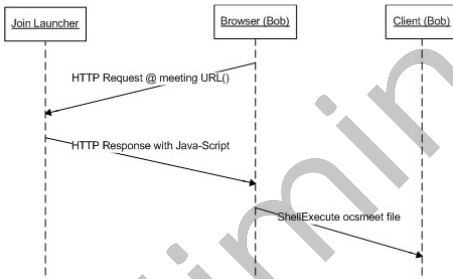
Figure 3: Simple Join
