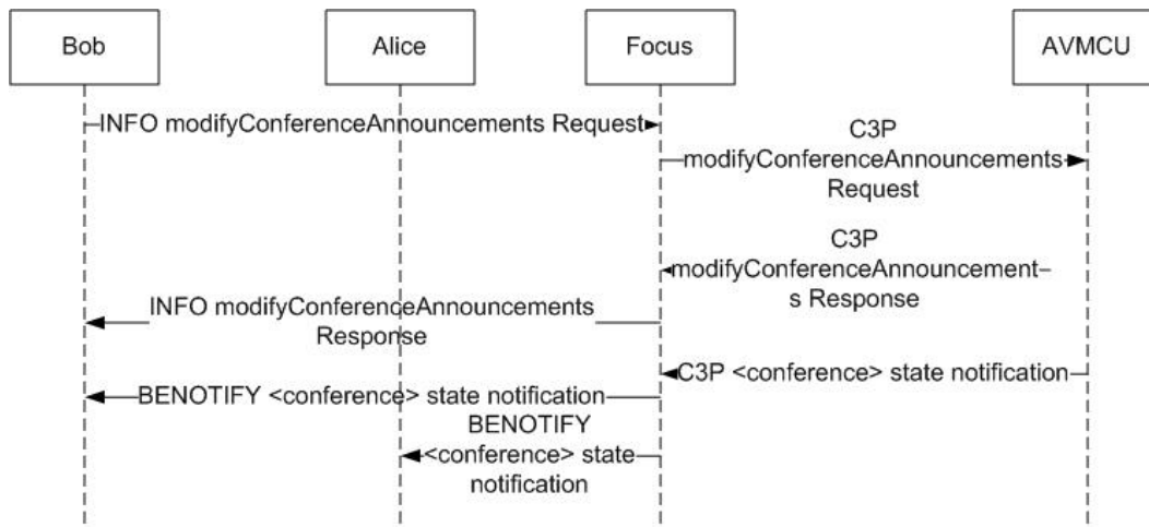
Figure 4: modifyConferenceAnnouncements message flow
