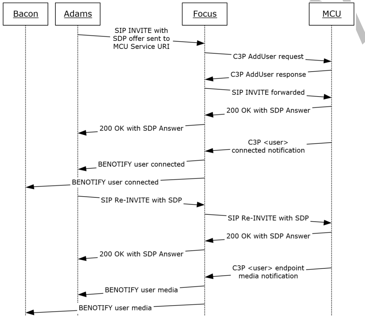
Figure 1: addUser dial-in call flow sequence
