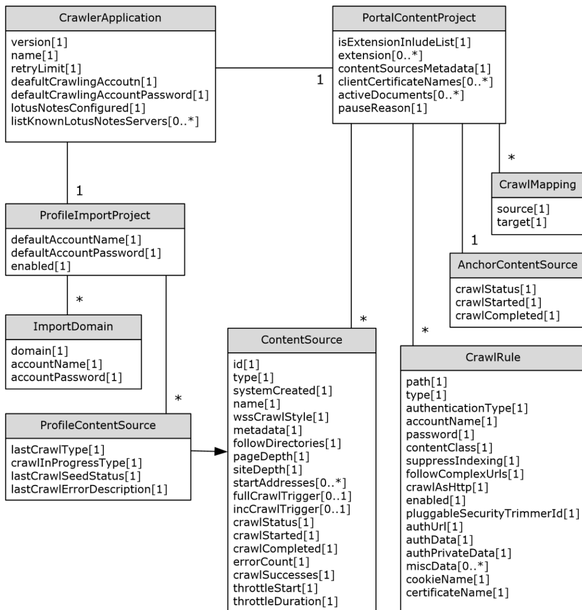
Figure 2: Object hierarchy
